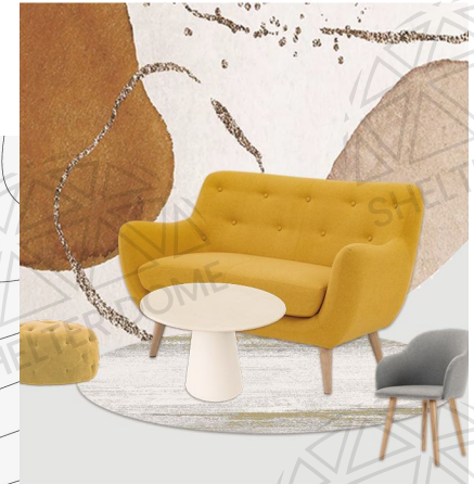
Multiplicity Variability
